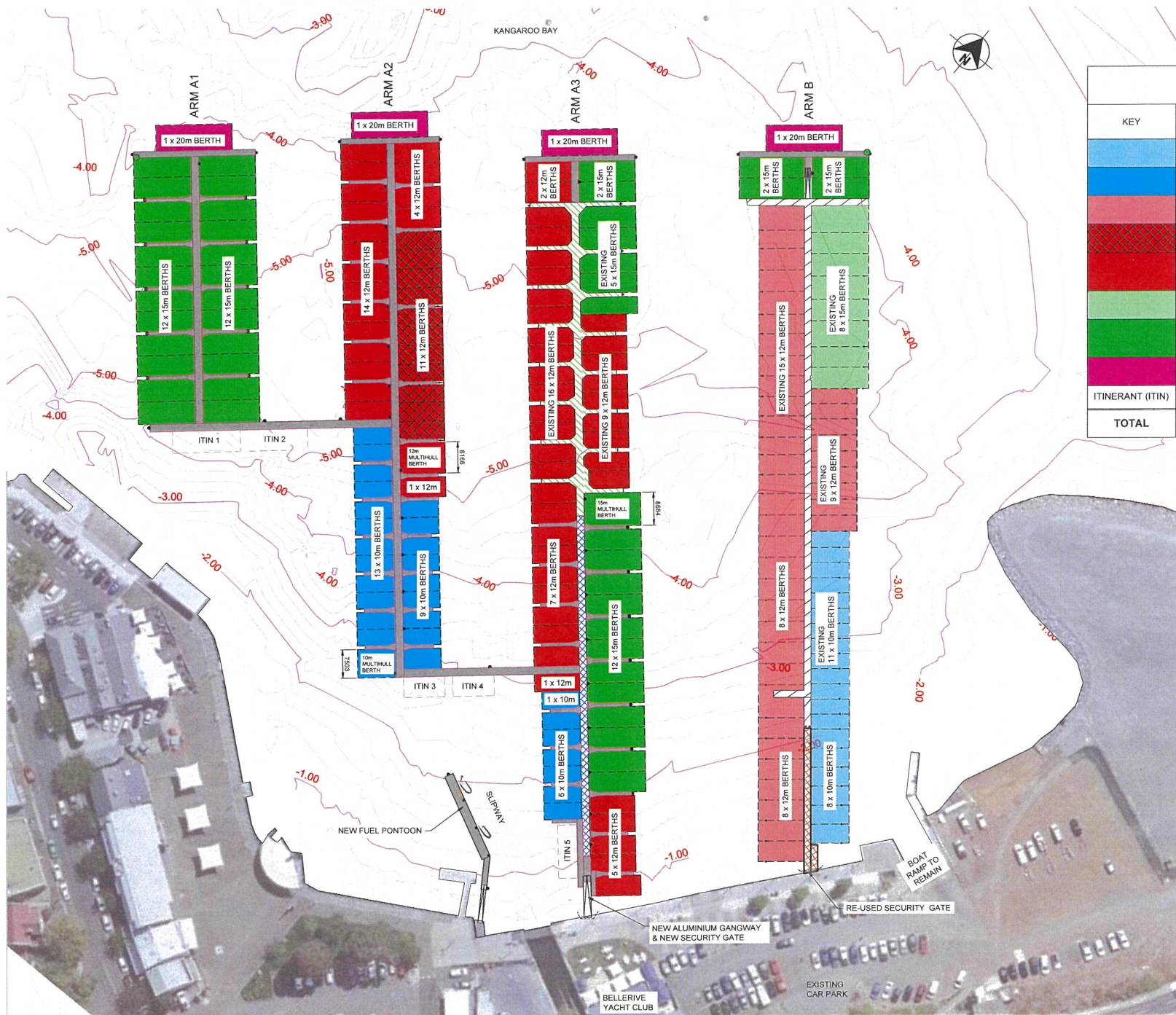
GENERAL ARRANGEMENT PLAN OF ALL BERTHS
